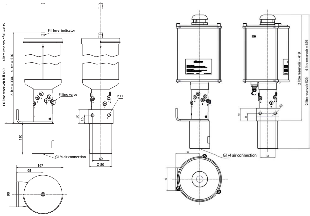
Metal reservoir
